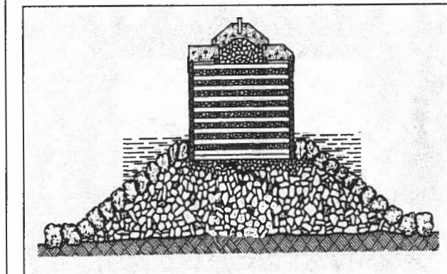
Typical stone-filled timber crib of the late 1800s, placed on an armor and core stone base (courtesy of U.S. Army Corps of Engineers).
