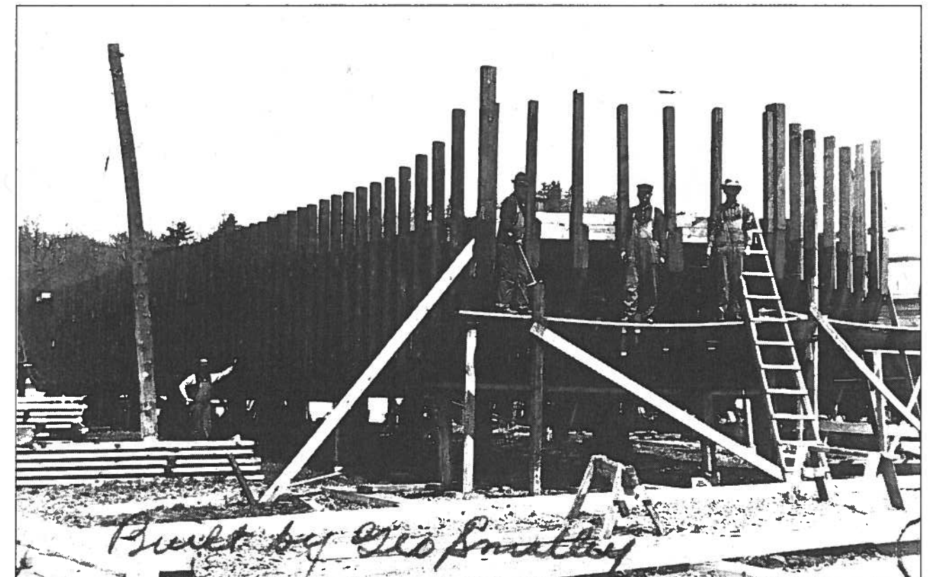
Unidentified scow schooner under construction at George Smalley Yards in Bay City, Michigan showing method for framing bow and sides (C. P. Labadie Collection).
