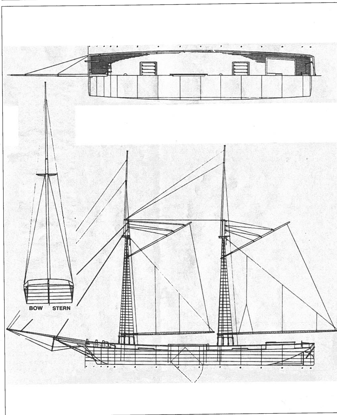
Modeler's plan of the 1867 scow schooner MILTON (artwork by James B. Jones, courtesy of Dossin Great Lakes Museum at Detroit, Michigan).
